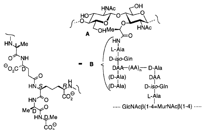
Figure 1. Typical primary structure of bacterial peptidoglycan (A); structure of the pentapeptide fragment (B); DAA = diamino acid [generally meso -diaminopimelic acid (as shown in B) or L-lysine]; (AA) n = n amino acids, with n = 0–5
