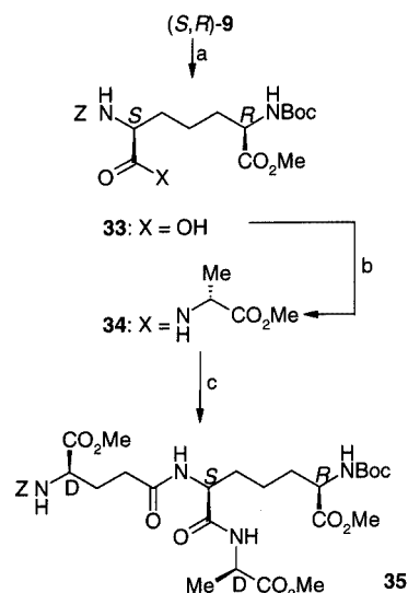
Scheme 6. Synthesis of peptide 35 ; a) TBAF, THF, room temp., IR 120, H + ; b) D-Ala(OMe), PyBOP, NMM, CH 2 Cl 2 (92%); c) Pd/C, H 2 , MeOH; Z-D-Glu-OMe, PyBOP, NMM, CH 2 Cl 2 (86%)
