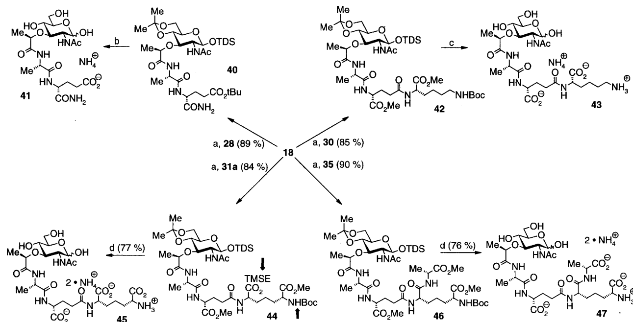
Scheme 9. Synthesis of muramyl peptides 41 , 43 , 45 , and 47 ; a) Pd/C, H 2 , MeOH; 28 , 30 , 31a , or 35 , Py BOP, NMM, CH 2 Cl 2 ; b) TFA/H 2 O/dioxane, 0 °C → room temp.; GPC (B-2 Biogel, NH 4 HCO 3 ); HPLC (H 2 O, MeCN, TFA); lyophilization (68%); c) LiOH, dioxane/H 2 O/MeOH, pH ≈ 10, room temp.; TFA/H 2 O/dioxane, 0 °C → room temp.; GPC (P-2 Biogel NH 4 HCO 3 ); HPLC (H 2 O, MeCN, TFA); lyophilization (64%); d) LiOH, dioxane/H 2 O/MeOH, pH ≈ 10, room temp.; TFA/H 2 O/dioxane, 0 °C → room temp.; GPC (P-2 Biogel, NH 4 HCO 3 ); lyophilization
