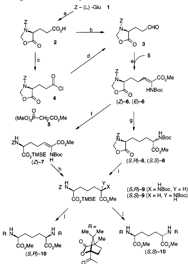
Scheme 1. Synthesis of diaminopimelic acid derivatives ( S,R )- 9 and ( S,S )- 9 ; a) (CH 2 O) m , toluene, Δ (86%); b) BH 3 ·SMe 2 , 0 °C \rightarrow room temp.; periodinane, room temp. (53%); c) SOCl 2 , Δ (76%); d) LiAl(O t Bu) 3 H, THF, −78 °C (73%); e) KHMDs, THF, −78 °C \rightarrow −30 °C [88%, ( Z )- 6 :( E )- 6 = 6.3:1]; f) Me 3 Si-CH 2 -CH 2 OH, LiHMDS, THF, 0 °C (65%); g) [RhCl(PPh 3 ) 3 ], H 2 , MeOH [90%, ( S,R )- 8 :( S,S )- 8 = 3:2]; h) Pd(OH) 2 /C, H 2 , MeOH; Z-Cl, NaHCO 3 , THF/H 2 O [70%, ( S,R )- 9 :( S,S )- 9 = 1:1]; i) TMSE-OH, LiHMDS, THF, 0 °C [70%, ( S,R )- 9 :( S,S )- 9 = 3:2]; j) 5 N HCl, 100 °C, 1 h; camphanoyl chloride, NaHCO 3 , THF/H 2 O; CH 2 N 2 , Et 2 O (65%)
