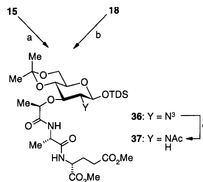
Scheme 7. Synthesis of muramic acid derivative 37 ; a) 29 , Pd/C, H 2 , MeOH; EEDQ, NEt 3 (65%); b) D-Glu(OMe) 2 , PyBOP, NMM, CH 2 Cl 2 ; c) H 2 S, Pyr, H 2 O; Ac 2 O, Pyr (85%)
