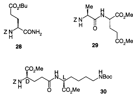
Scheme 4. Building blocks 28–30
