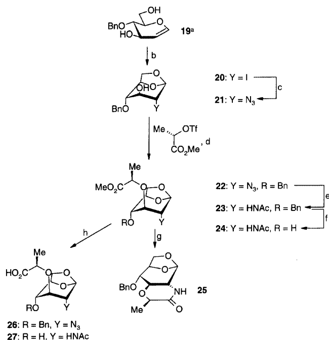
Scheme 3. Synthesis of 1,6-anhydroneuramic acid derivatives 26 and 27 ; a) ref. 28; b) (Bu 3 Sn) 2 O, MeCN, Δ; I 2 , room temp. (89%); c) TMGA, DMF, H 2 O, Δ, 3 days (79% + 15% manno isomer); d) NaH, CH 2 Cl 2 (85–88%); e) H 2 S, pyr/H 2 O; Ac 2 O, pyr (92%); f) Pd/C, H 2 ; Ac 2 O; MeOH (90%); g) PPh 3 , THF/H 2 O; Ac 2 O, pyr (75%); h) LiOH, dioxane/MeOH (quant.)
