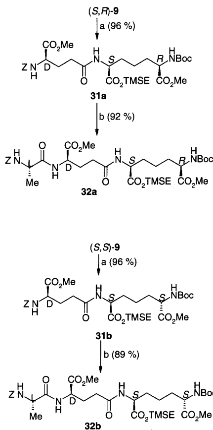
Scheme 5. Synthesis of peptides 32a and 32b ; a) Pd/C, H 2 , MeOH; Z-D-Glu-OMe, PyBOP, NMM, CH 2 Cl 2 ; b) Pd/C, H 2 , MeOH; Z-L-Ala, PyBOP, NMM, CH 2 Cl 2
