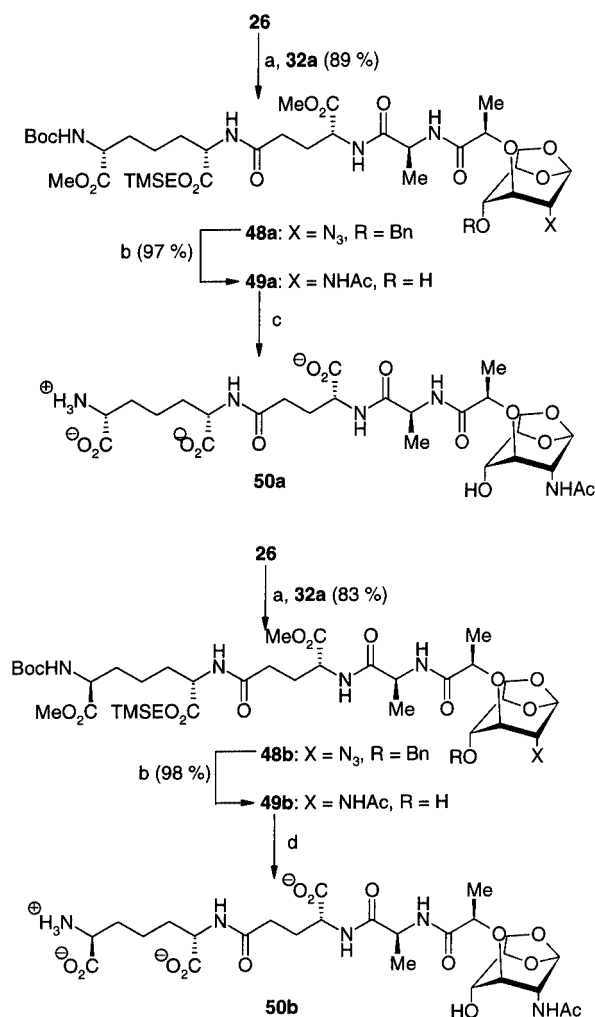
Scheme 10. Synthesis of 1,6-anhydromuramylpeptides 50a and 50b : a) Pd/C, H 2 , MeOH; Py BOP, NMM, DMF; b) Pd/C, H 2 , MeOH; Ac 2 O; c) TFA, CH 2 Cl 2 , room temp.; LiOH, H 2 O/MeOH, pH ≈ 10, room temp.; Dowex 50 W; RP-18 (MeCN/H 2 O); lyophilization (86%); d) TFA, CH 2 Cl 2 , room temp.; LiOH, H 2 O/MeOH, pH ≈ 10, room temp.; Dowex 50 W; RP-18 (MeCN/H 2 O); Dowex 50 W; lyophilization (77%)
