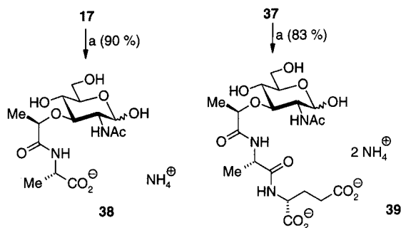
Scheme 8. Synthesis of muramic acid derivatives 38 and 39 ; a) LiOH, dioxane/MeOH/H 2 O, room temp., pH 9.5–10.5; TFA/H 2 O/dioxane, 0 °C → room temp.; GPC (P 2 -Biogel, NH 4 HCO 3 ) lyophilization
